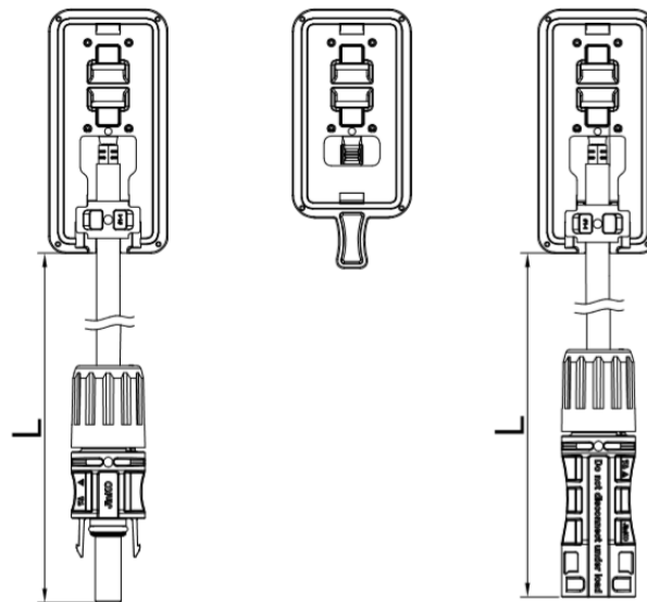
Fig. 13 (2) The half-cut cell module/ split junction box
